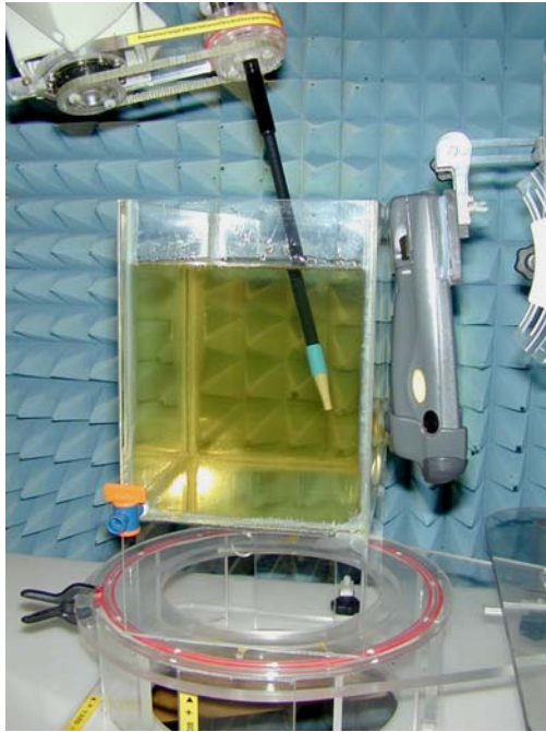
Figure 34. Positional photograph of PDT8056 in the Touch Position 900MHz Fluid
