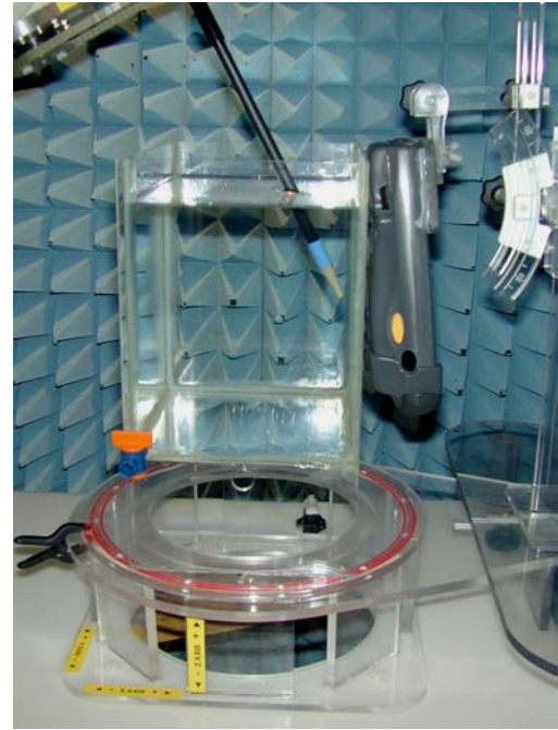
Figure 35. Positional photograph of PDT8056 in the Touch Position for 1800/1900/2450 MHz Fluids
