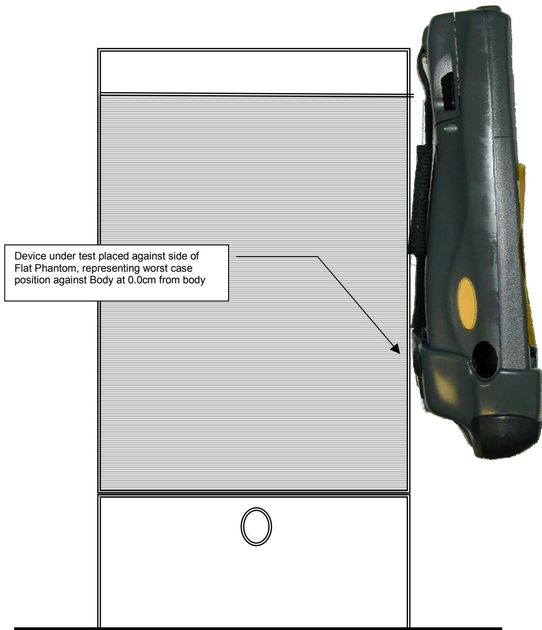
Figure 17. – Touch Position; to demonstrate worst case test position.
