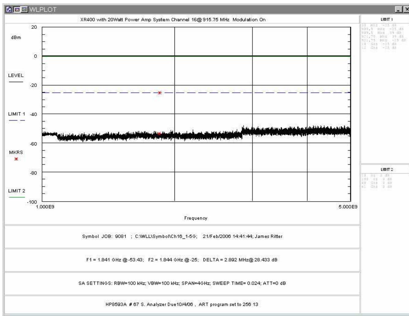
Figure 4-14. Conducted Spurious Emissions, Channel 16: 1 –5GHz
