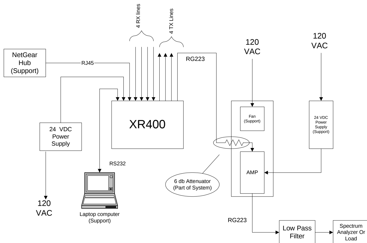
Figure 2-1. Test Configuration.
