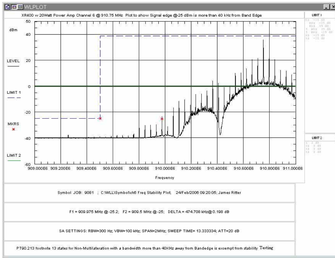
Figure 4-16, Frequency Stability Plot Showing >40kHz from Bandedge, Low Channel
