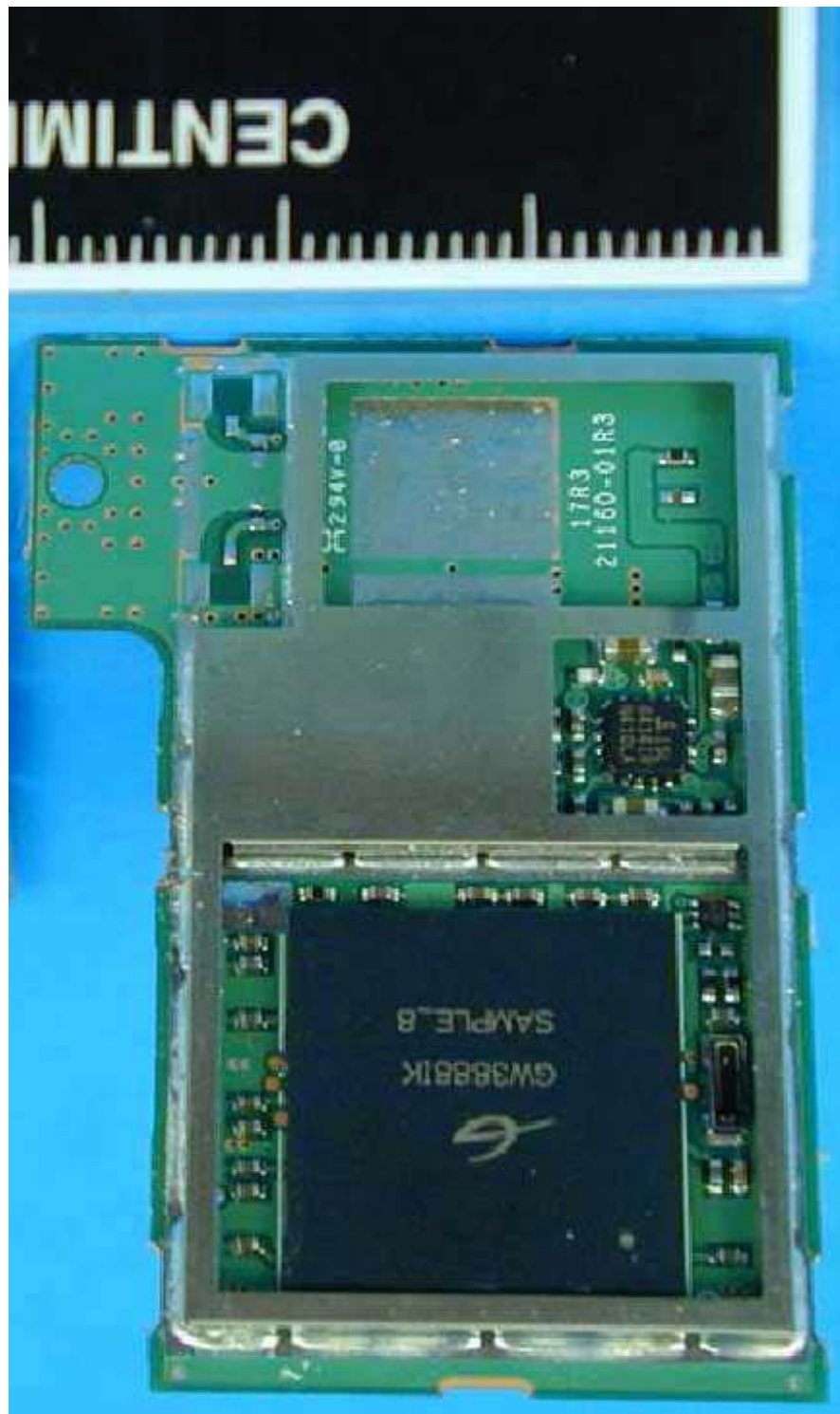
WLAN (802.11a/b/g) Module (With RF Shield Removed)
