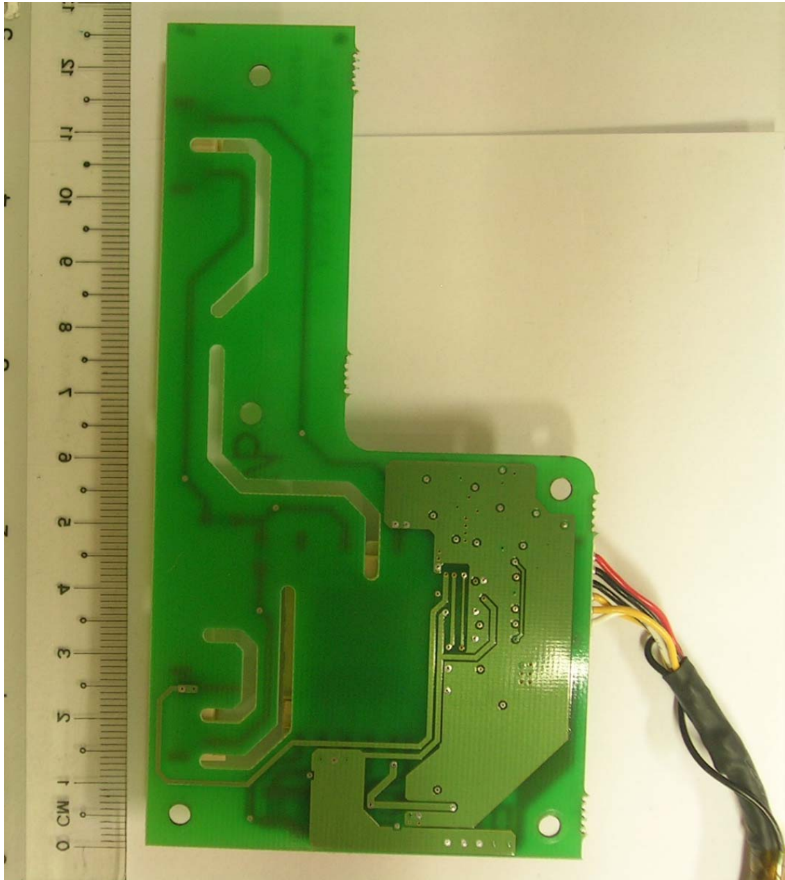
PCB Trace Side - LCD Display Board
