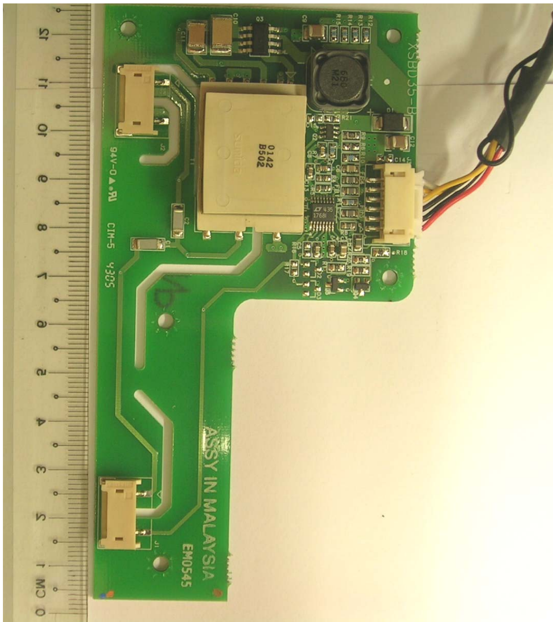
PCB Component Side - LCD Display Board
