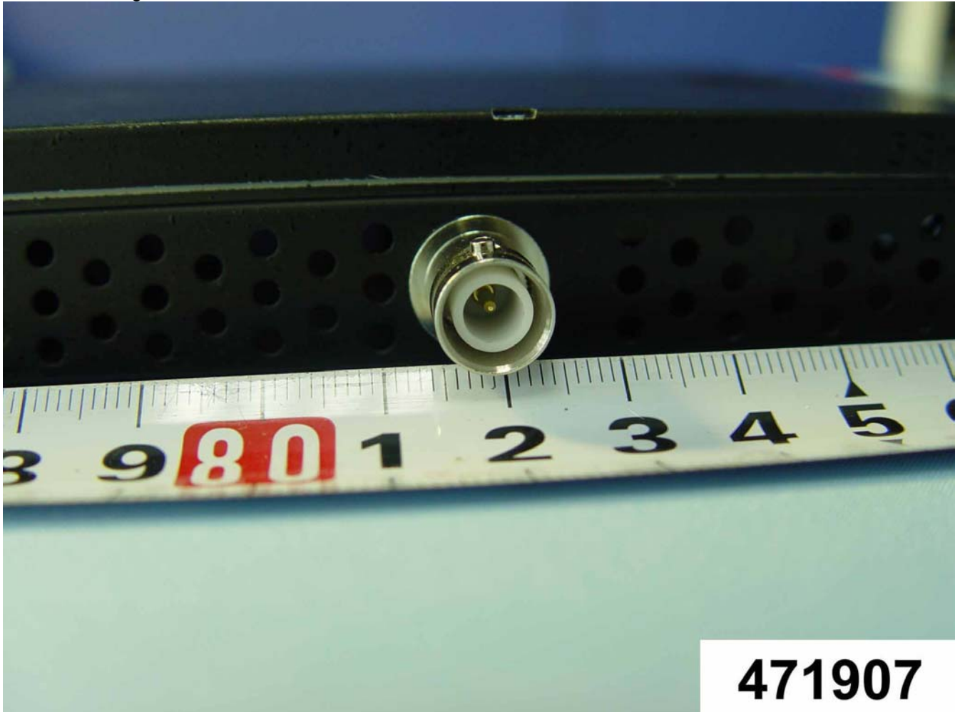
Metallic Housing
