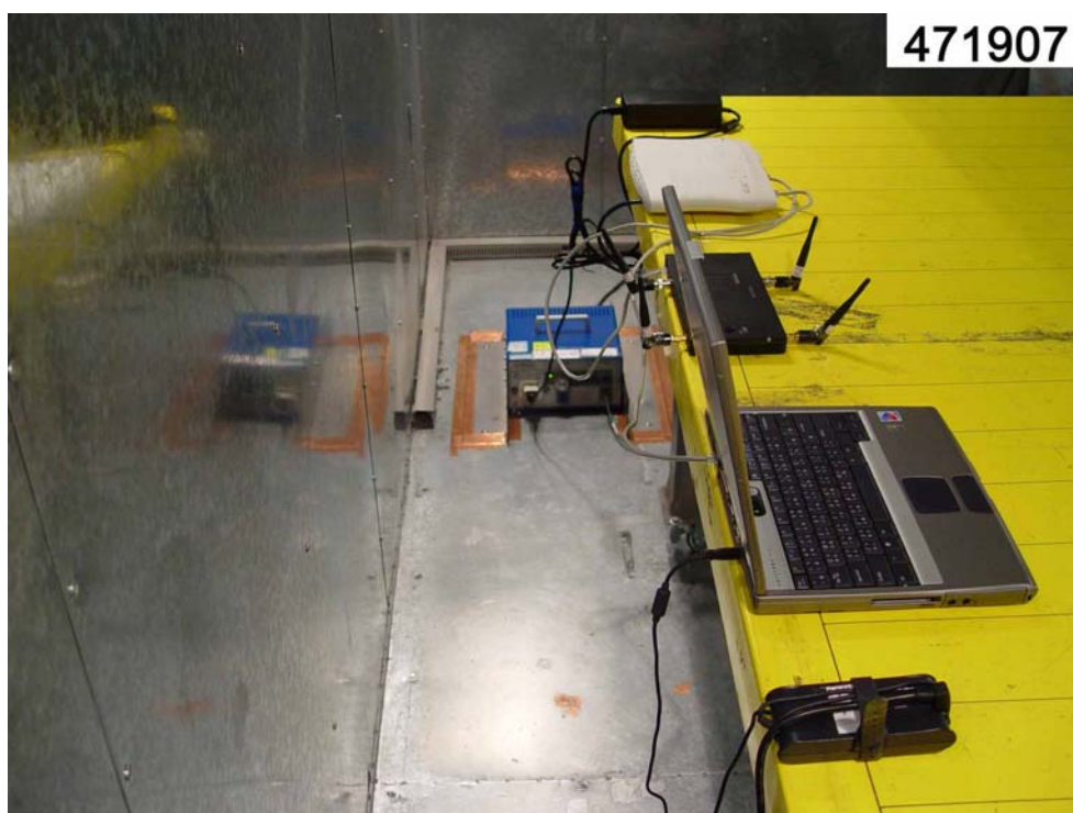
REAR VIEW (Metallic Housing WASP-5100)
