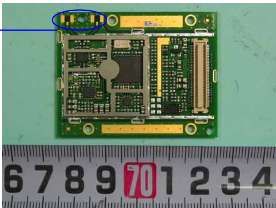
Bluetooth Antenna Location
