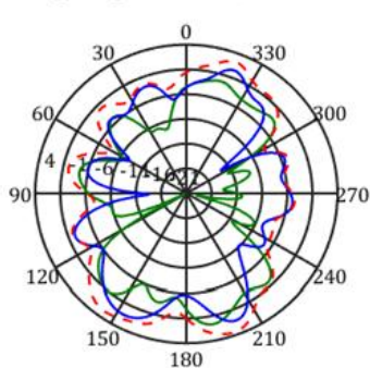
frequency=2450MHz, X-Y Plane
