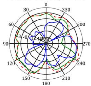
frequency=2450MHz, Y-Z Plane
