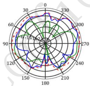
frequency=2450MHz, X-Z Plane
