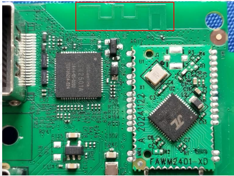
BT Antenna
