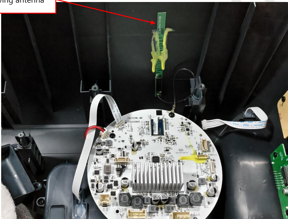
FM receiving antenna
