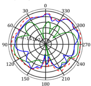
frequency=2450MHz, X-Z Plane
