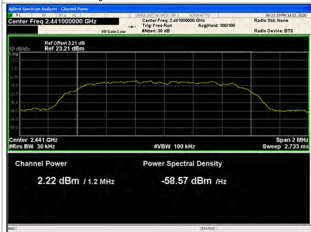
Average Power NVNT 3-DH5 2441MHz Ant1
