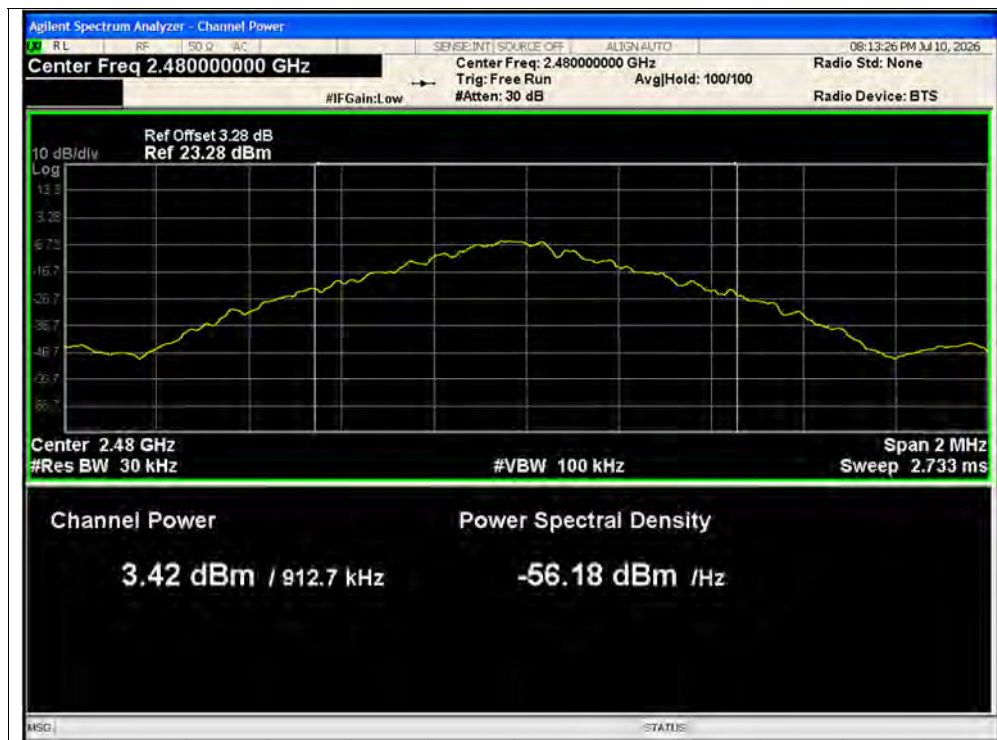
Average Power NVNT 1-DH5 2480MHz Ant1
