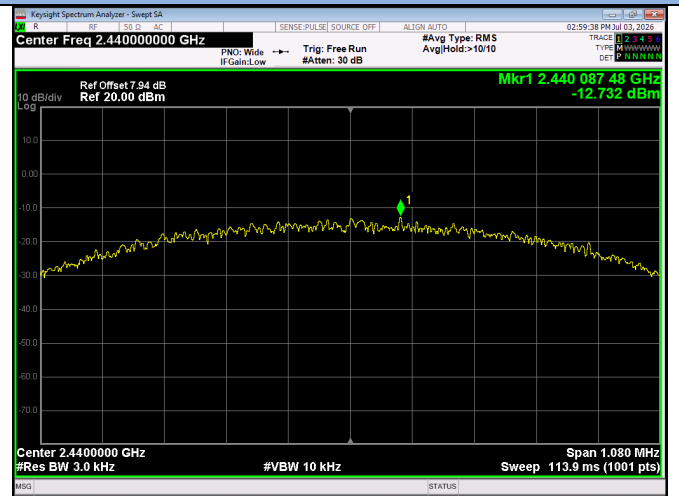
RF PHY 1Mbps 2440MHz
