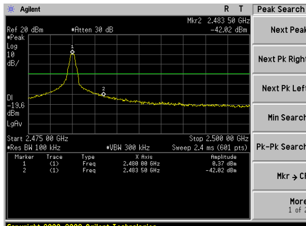
BDR mode (GFSK): Band Edge-High Channel
