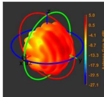
frequency=2450MHz, X-Y Plane
