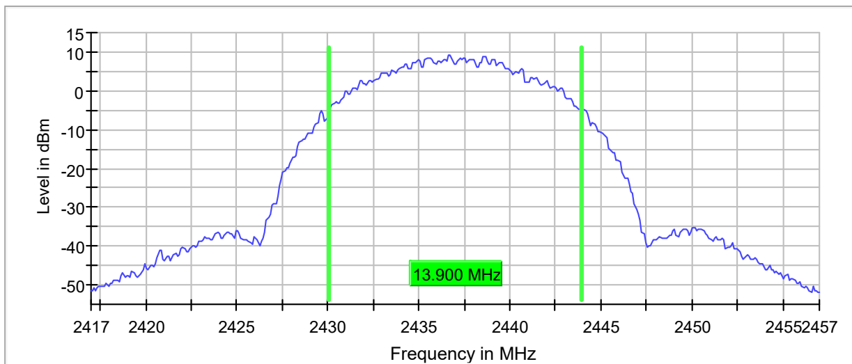
99 % Bandwidth
