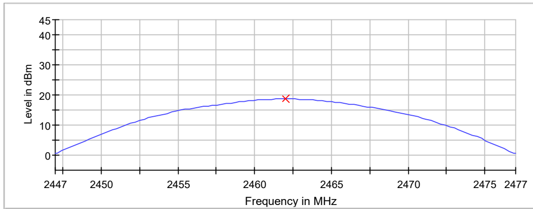
Peak Power
