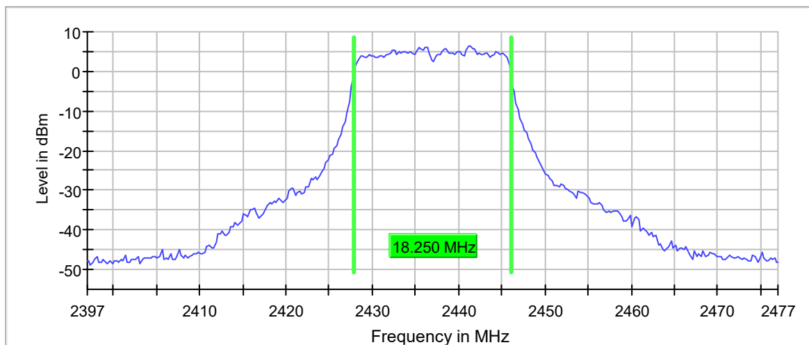
99 % Bandwidth
