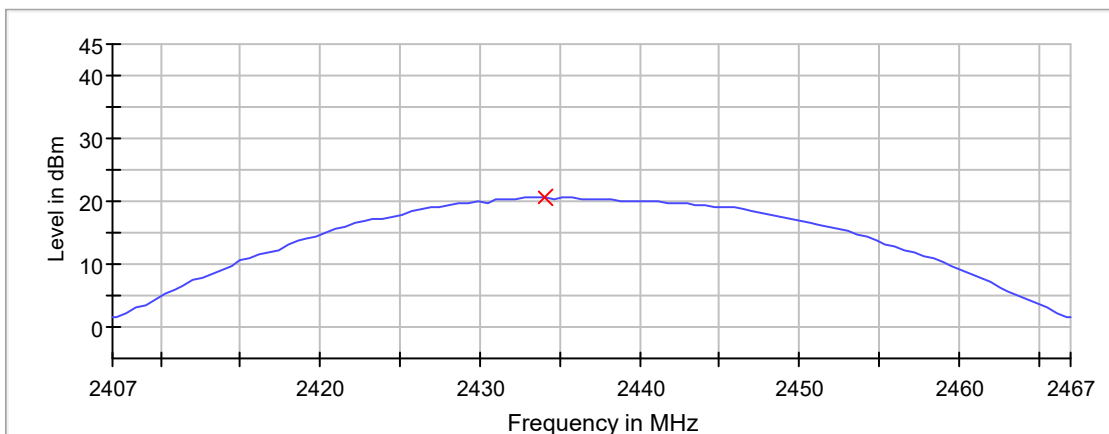
Peak Power
