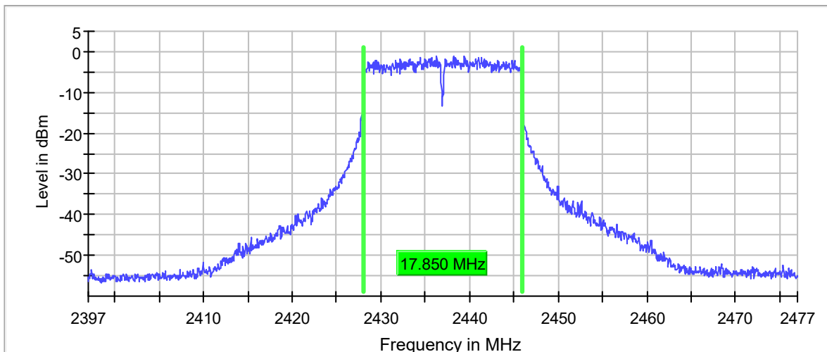
6 dB Bandwidth
