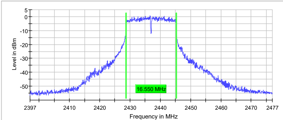
6 dB Bandwidth
