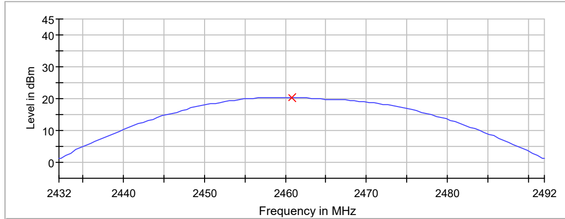
Peak Power
