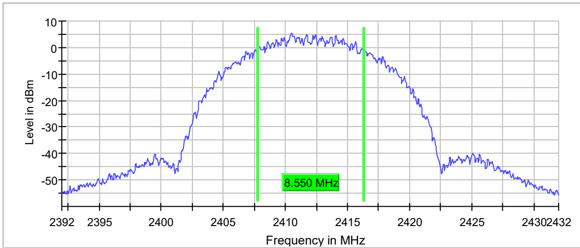
6 dB Bandwidth
