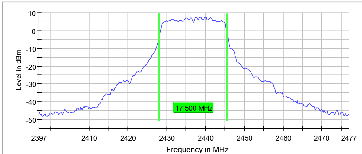
99 % Bandwidth
