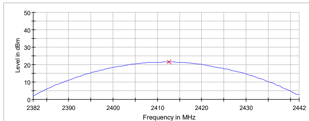
Peak Power
