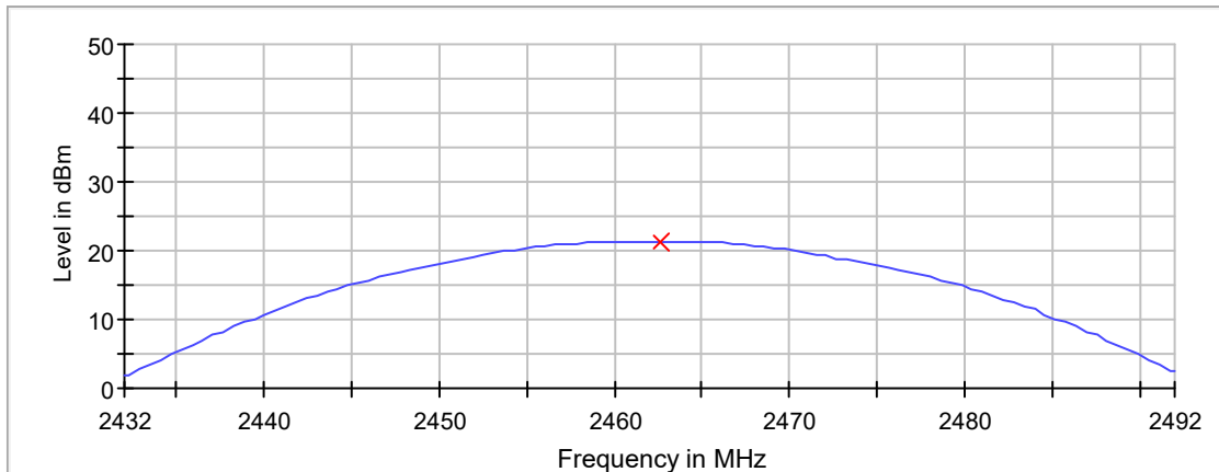
Peak Power
