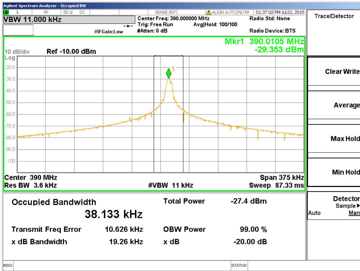
Figure 20 – 99% Bandwidth Graph
