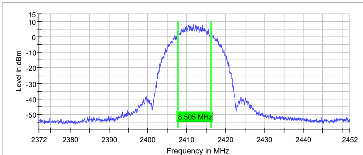
6 dB Bandwidth
