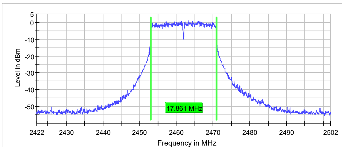
6 dB Bandwidth
