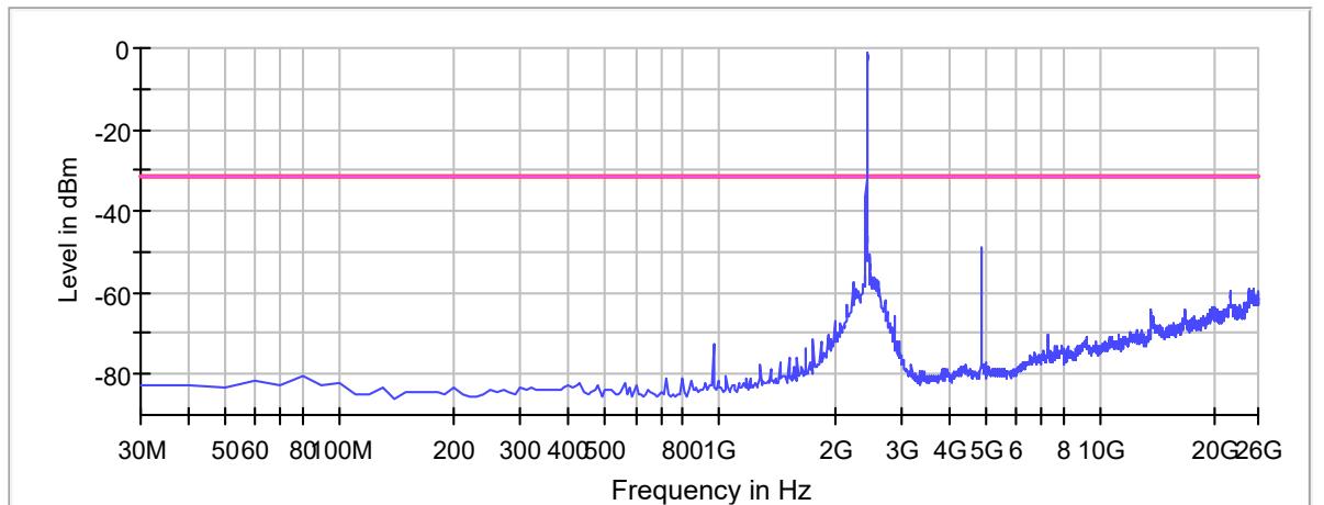
Spurious
