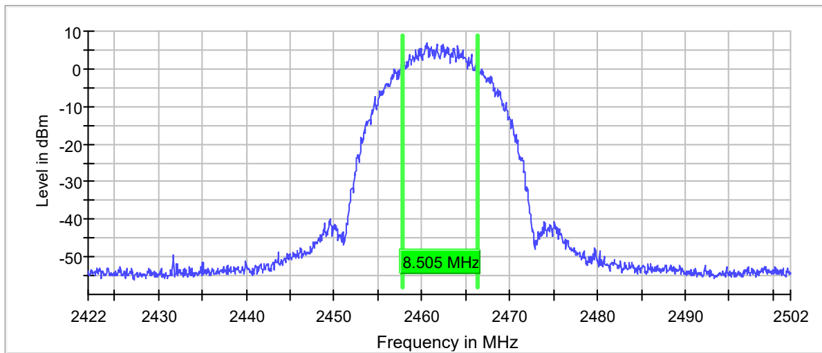
6 dB Bandwidth
