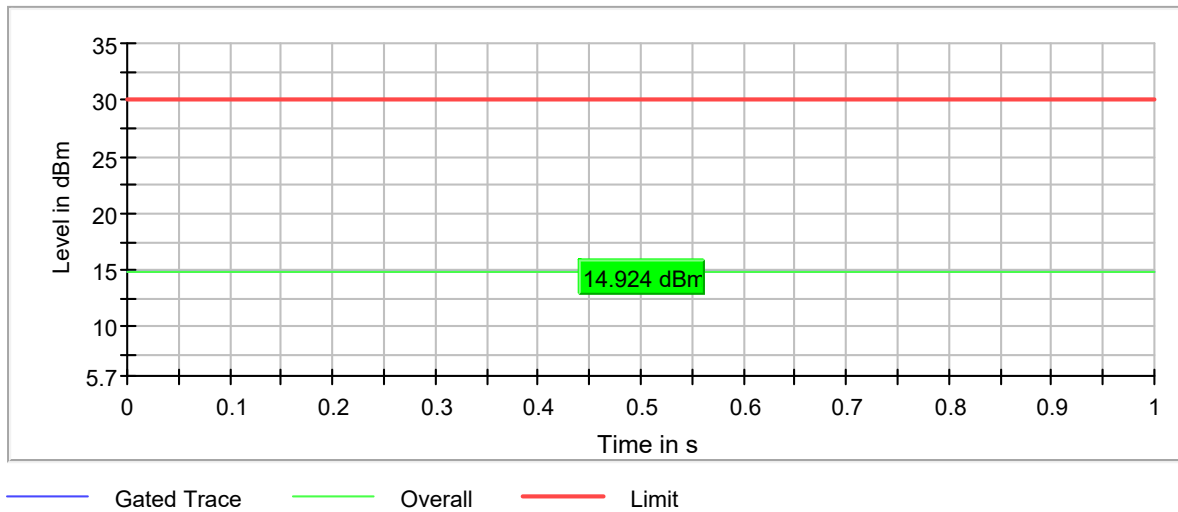
Gated Trace
