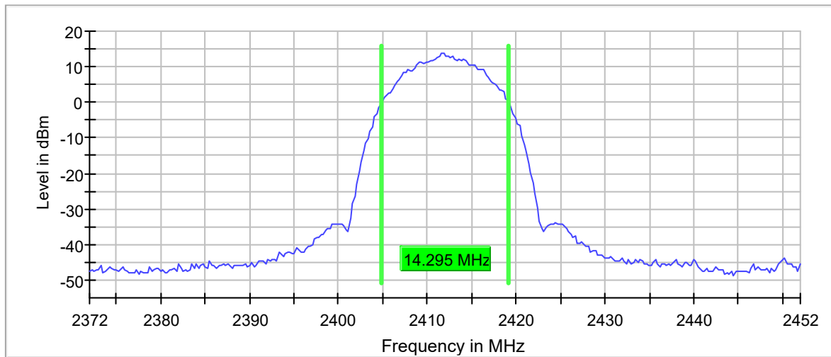
99 % Bandwidth
