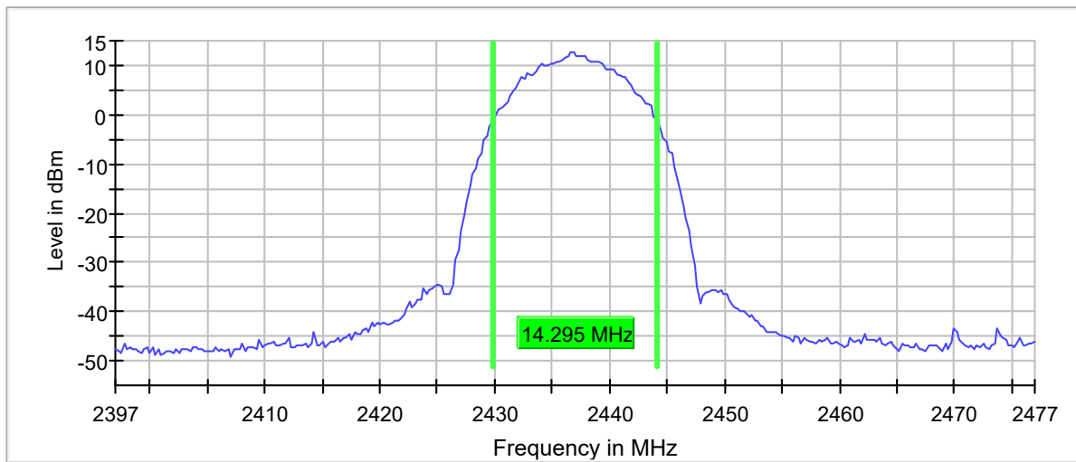
99 % Bandwidth
