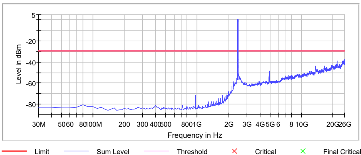
Spurious
