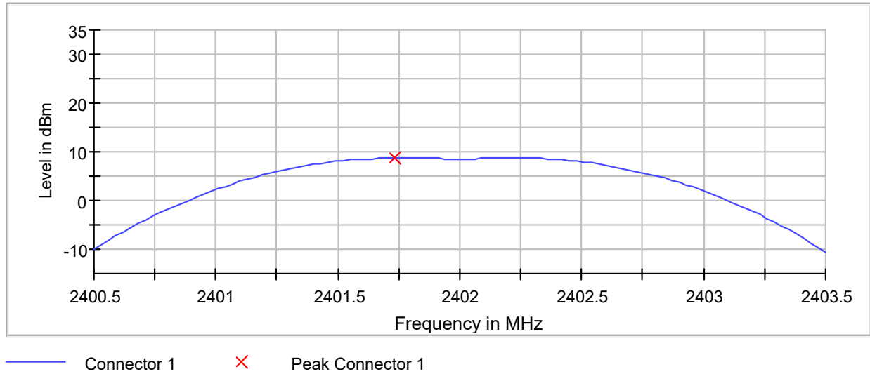
Peak Power
