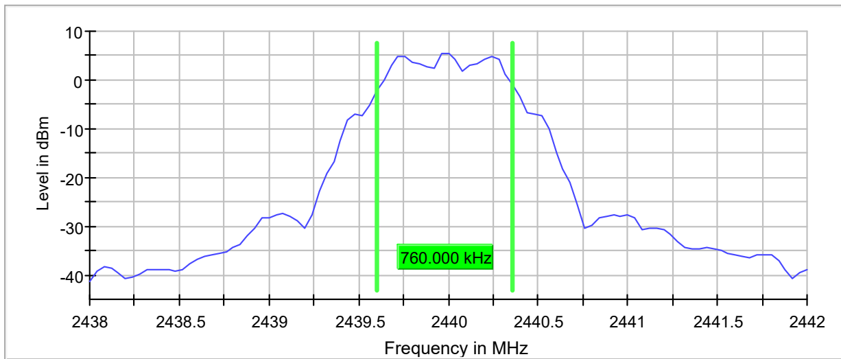
6 dB Bandwidth
