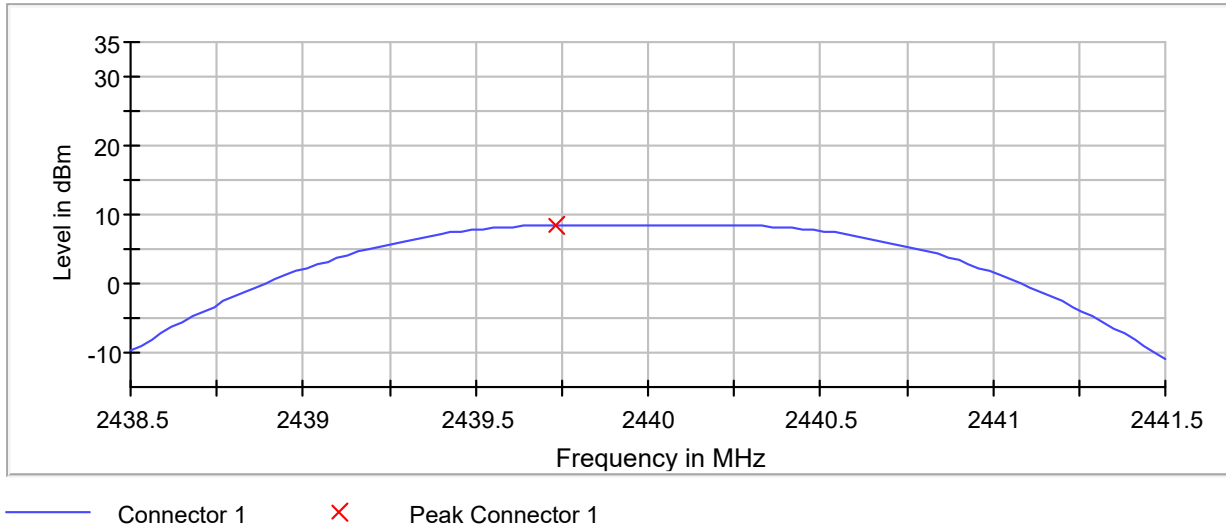
Peak Power
