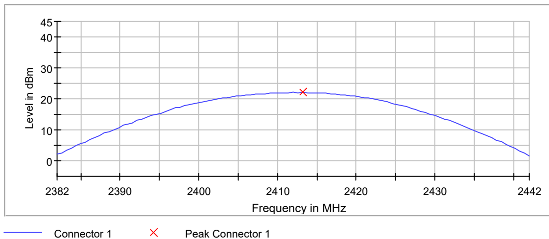
Peak Power
