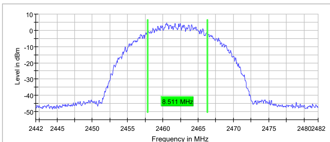
6 dB Bandwidth
