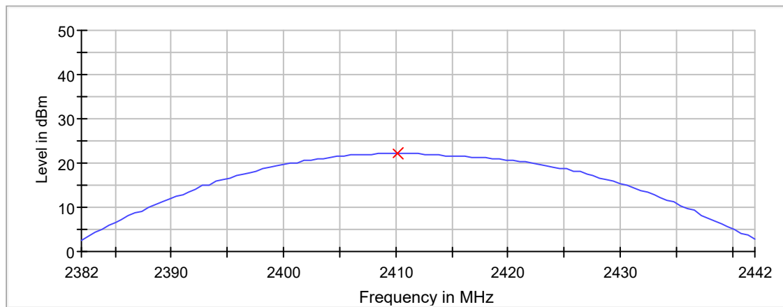
Peak Power
