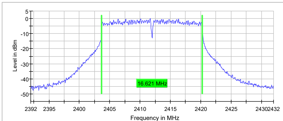
6 dB Bandwidth
