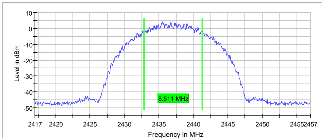
6 dB Bandwidth
