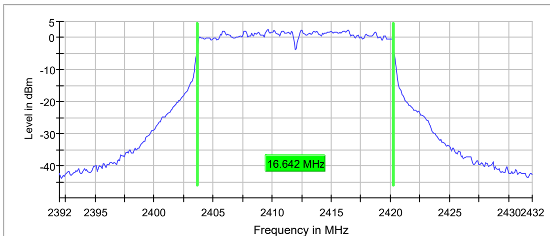
99 % Bandwidth
