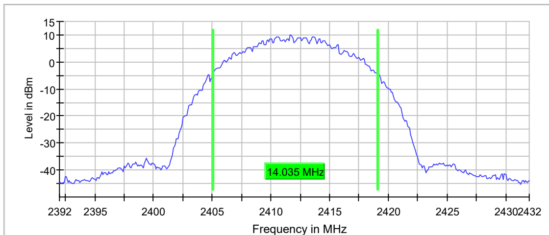
99 % Bandwidth
