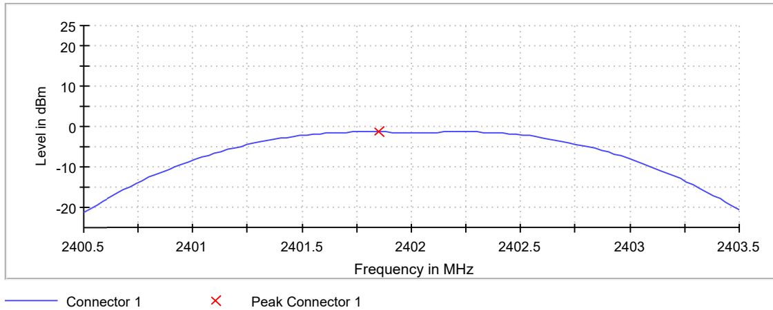
Peak Power
