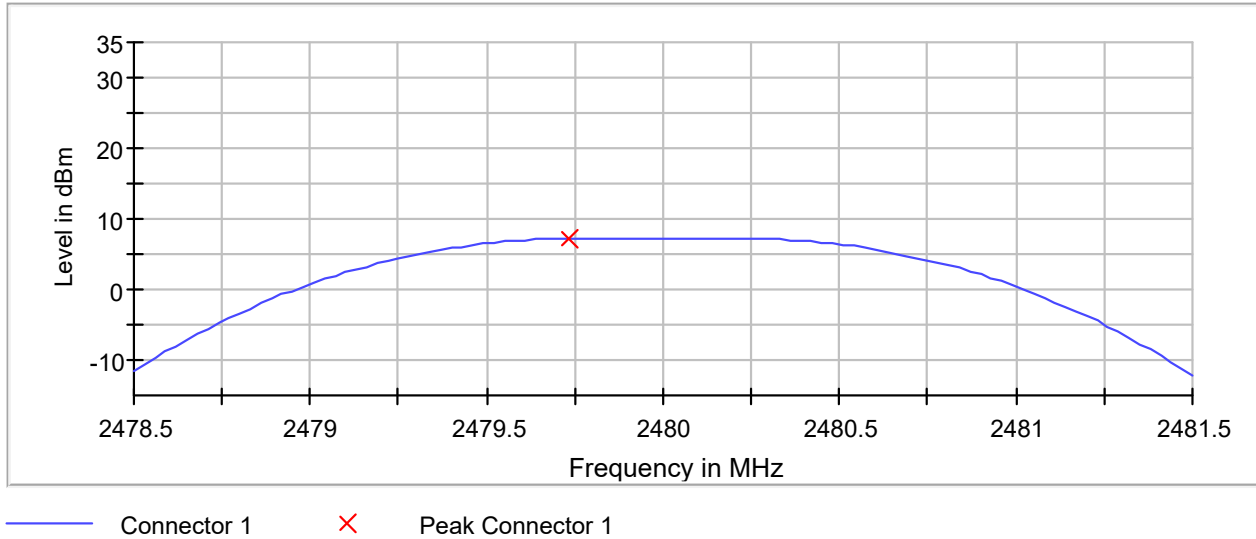
Peak Power
