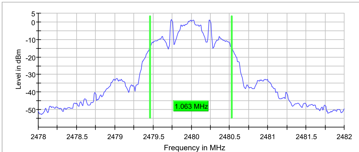
99 % Bandwidth
