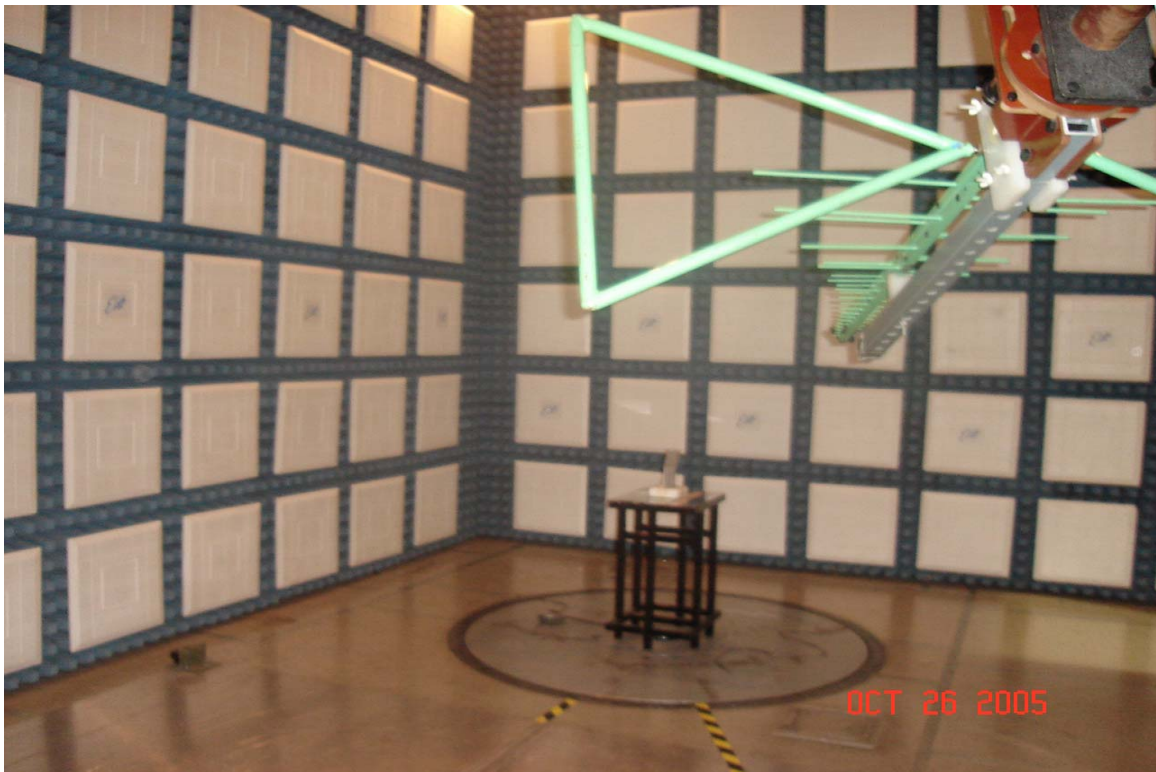
Test Set-up for Radiated Emissions Horizontal Polarization
