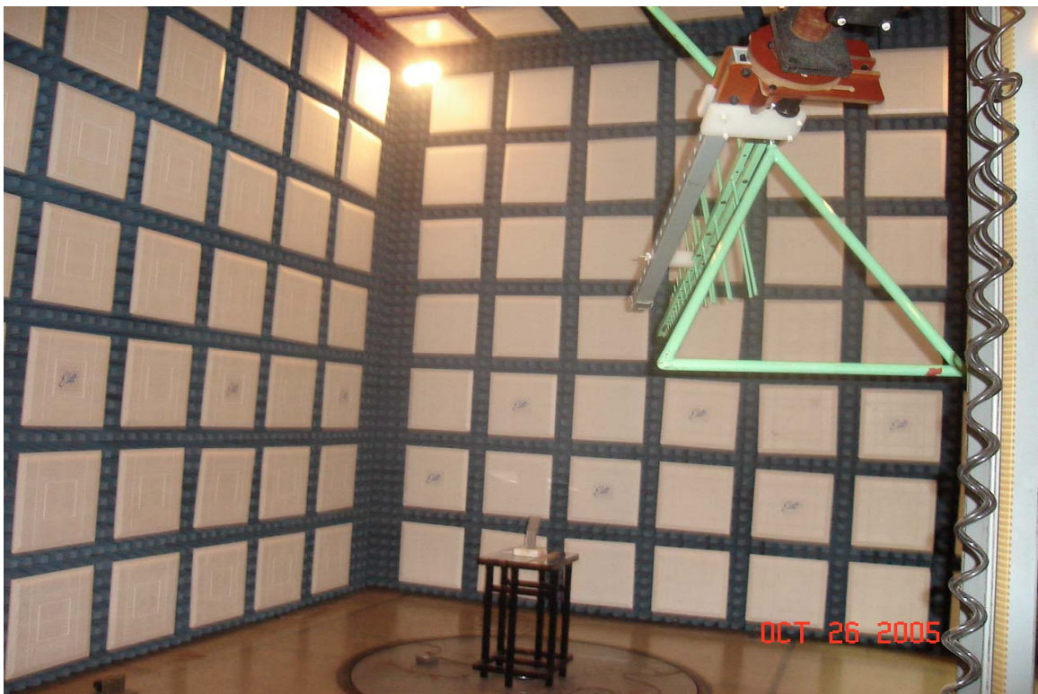
Test Set-up for Radiated Emissions Vertical Polarization
