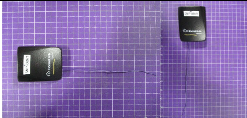
8 inch 18 gauge dipole wire antenna.
