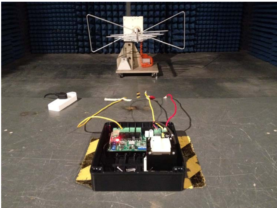
Radiated Emission
