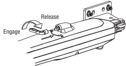
The clutch release for the right operator
