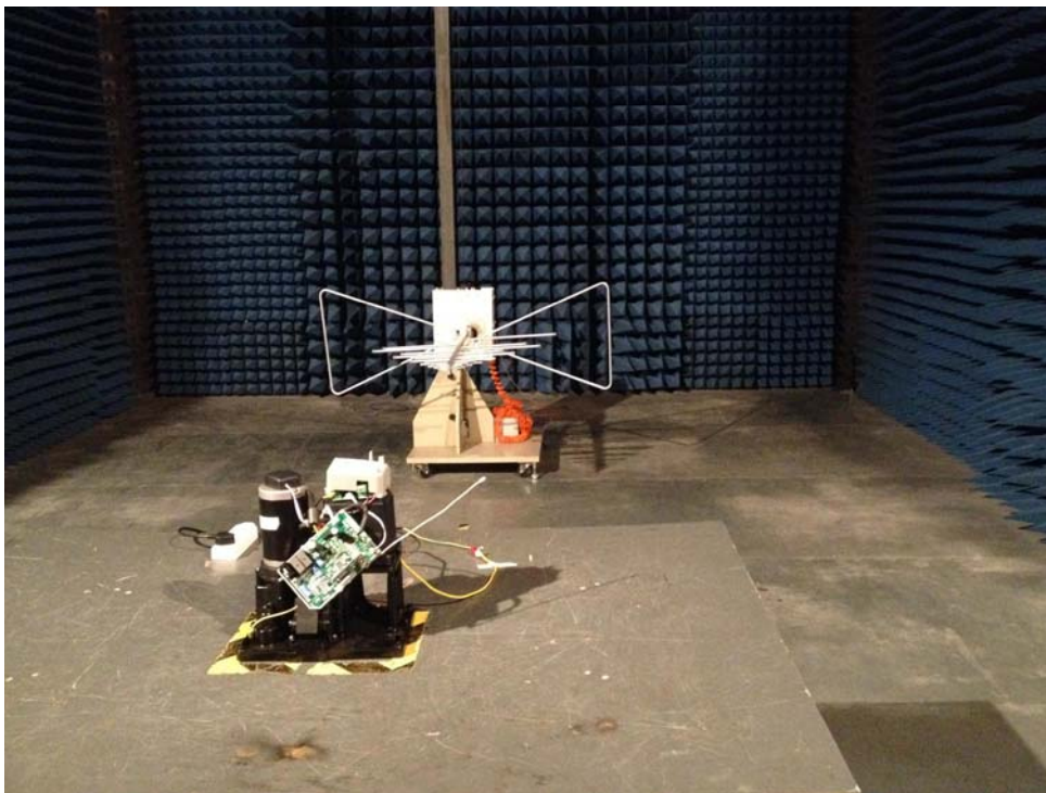
Radiated Emission
