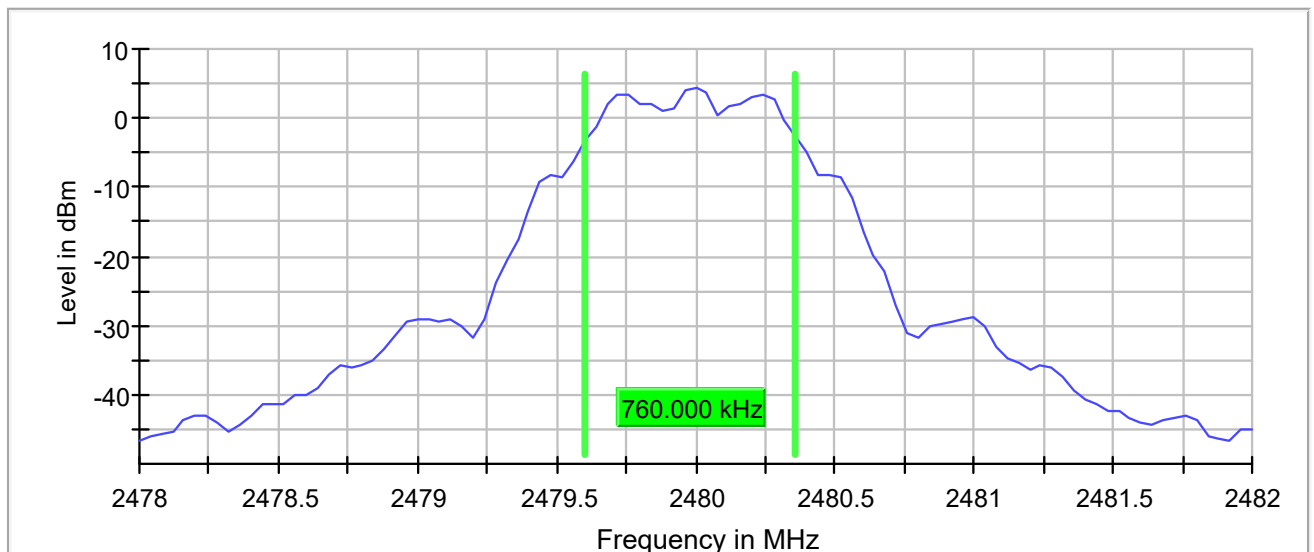
6 dB Bandwidth
