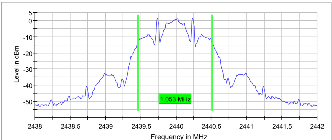
99 % Bandwidth
