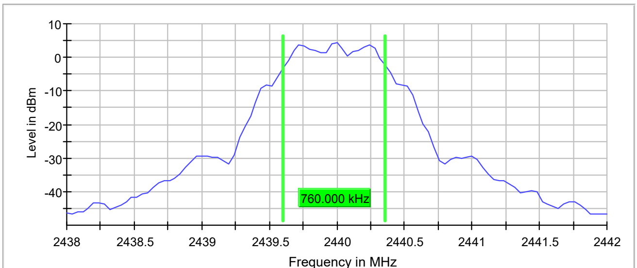
6 dB Bandwidth
