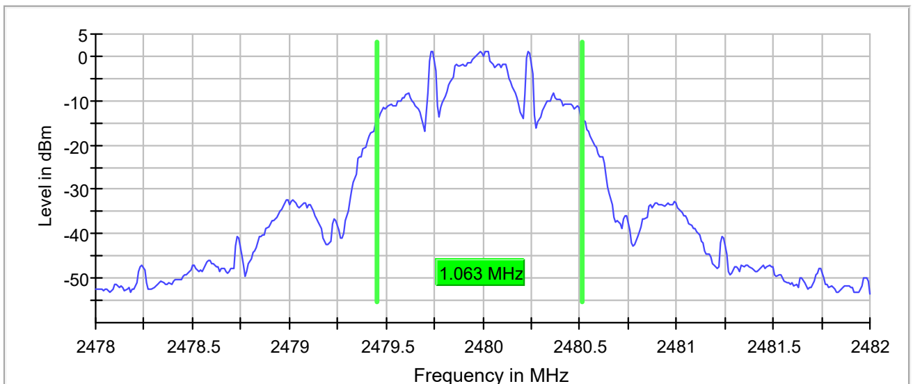
99 % Bandwidth
