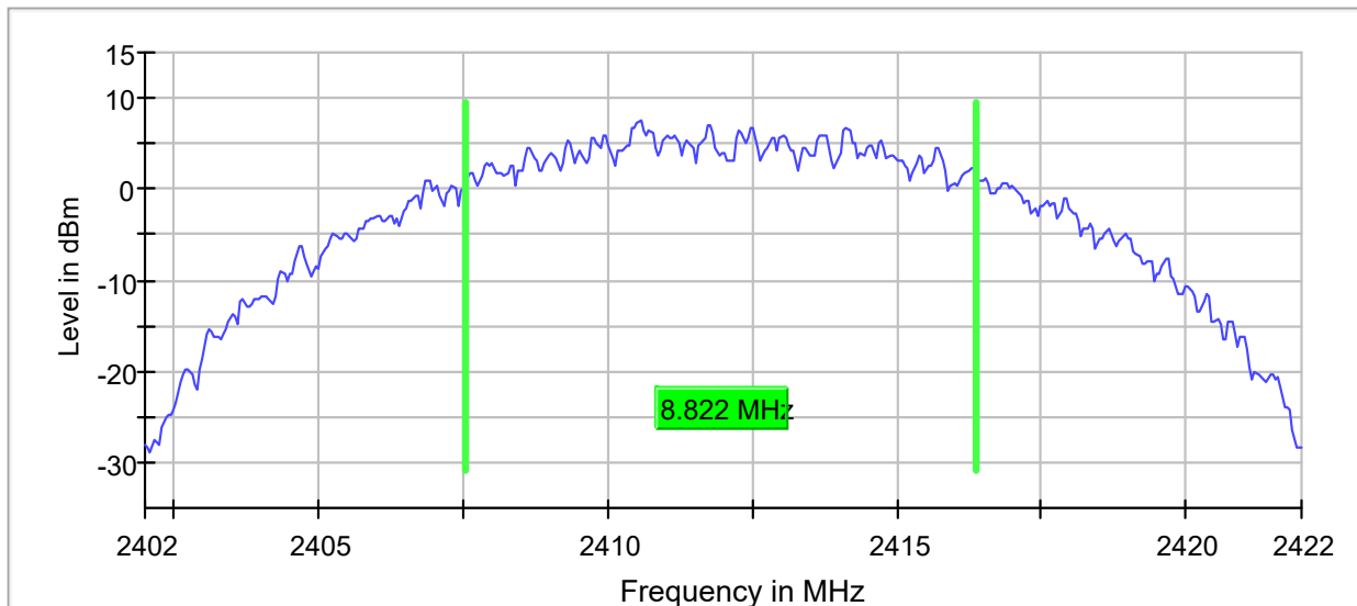
6 dB Bandwidth
