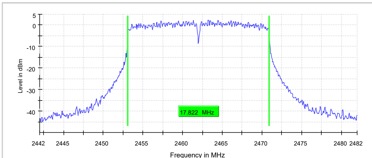
6 dB Bandwidth
