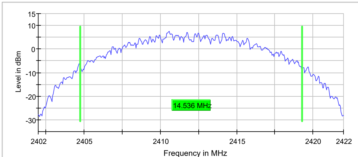
99 % Bandwidth
