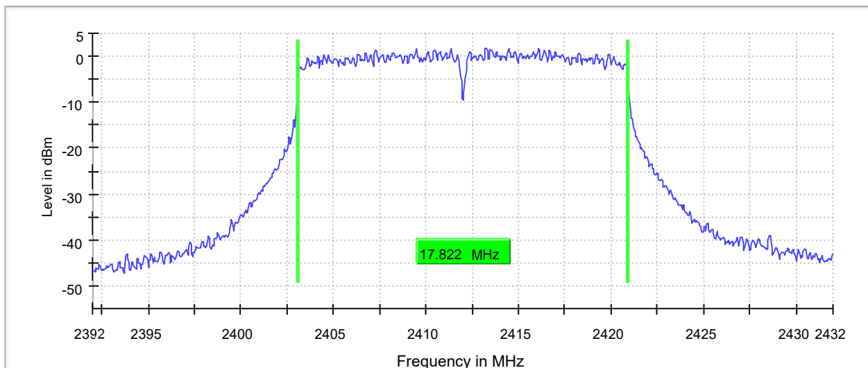
6 dB Bandwidth
