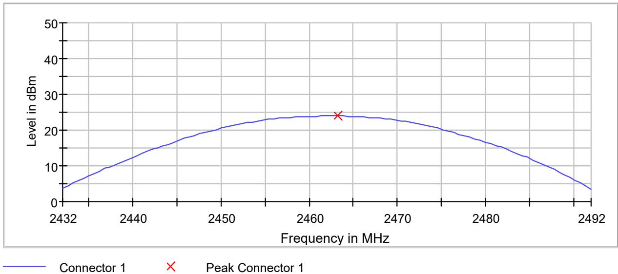
Peak Power
