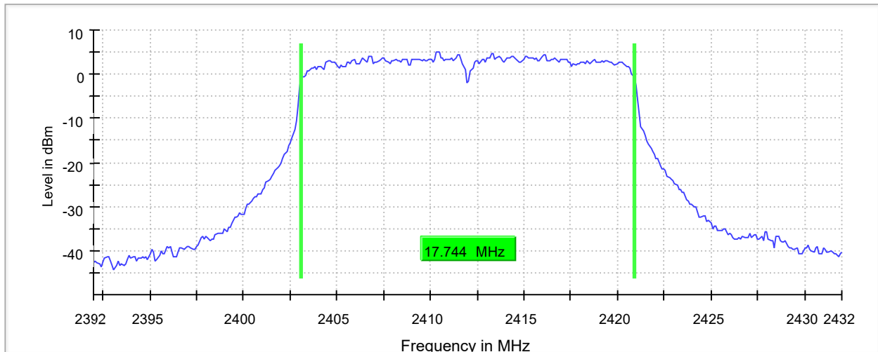
99 % Bandwidth
