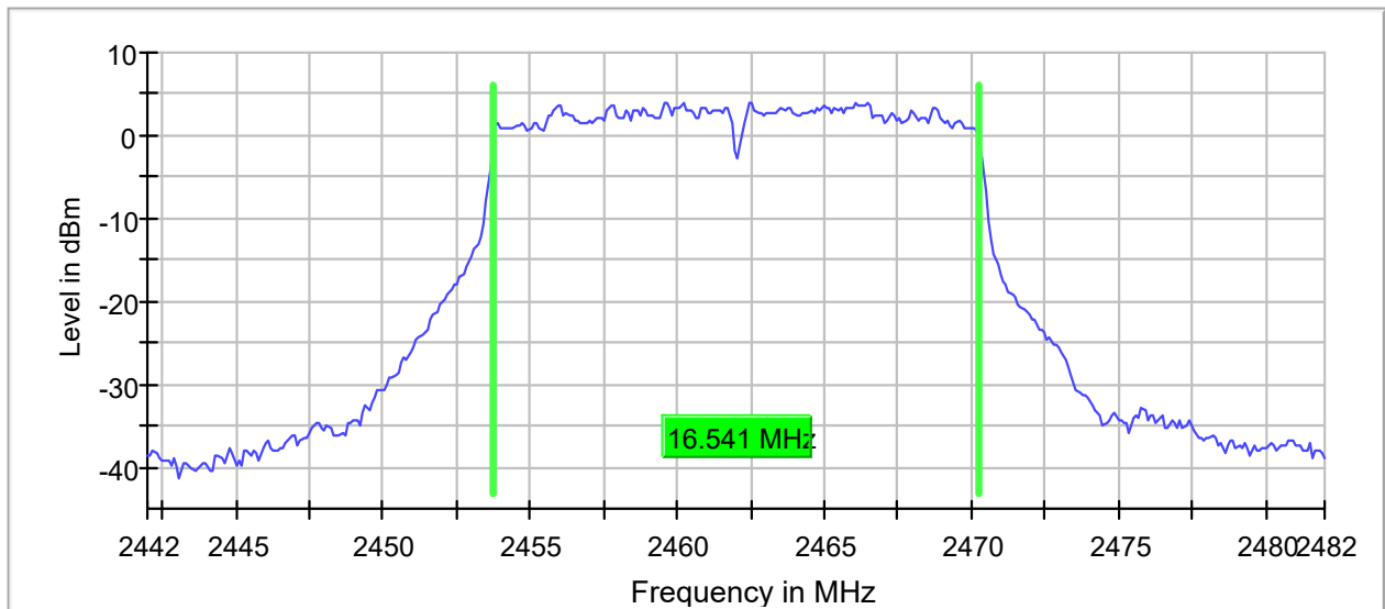
99 % Bandwidth
