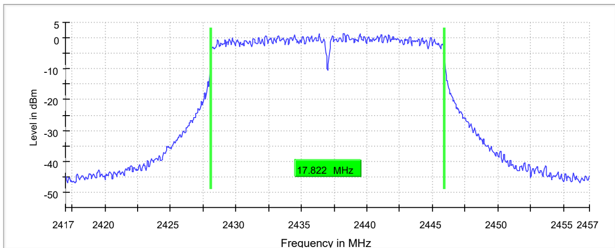
6 dB Bandwidth
