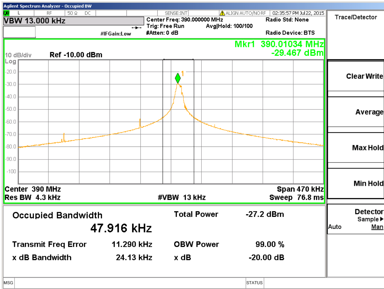
Figure 8 – 99% Bandwidth Graph
