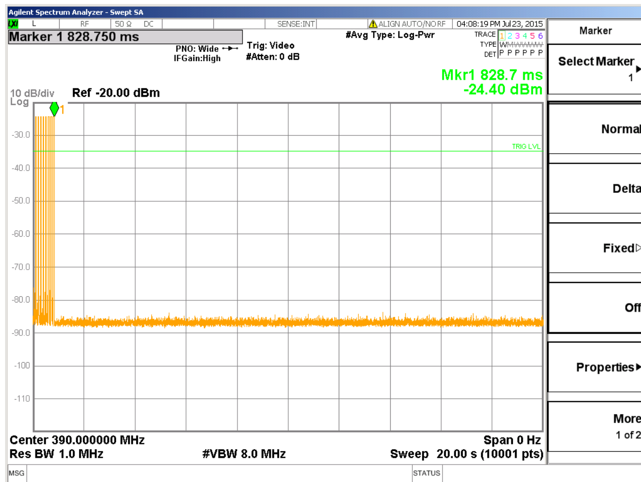
Figure 51 Cease Operation Graph 390MHz
