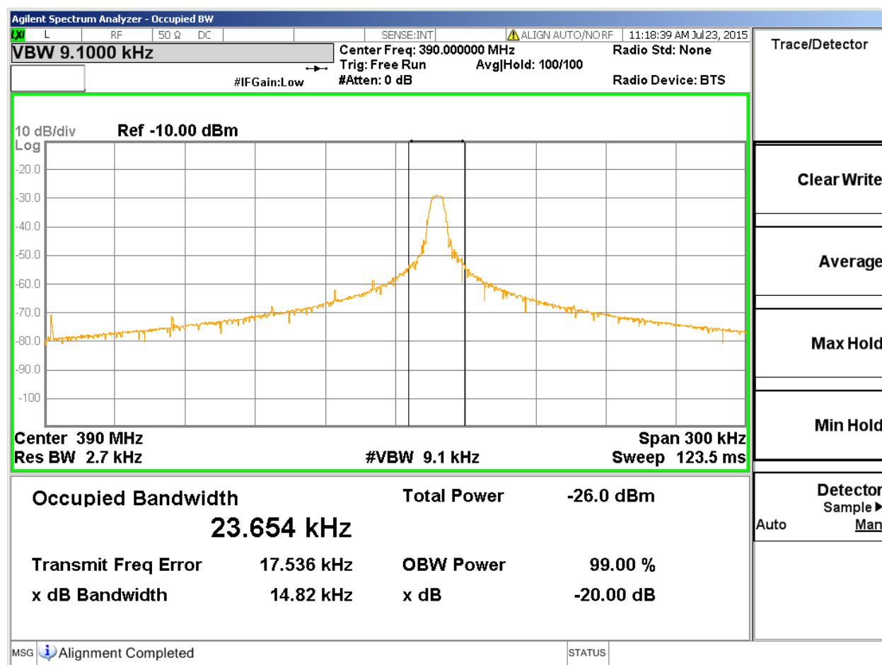
Figure 32 – 99% Bandwidth Graph
