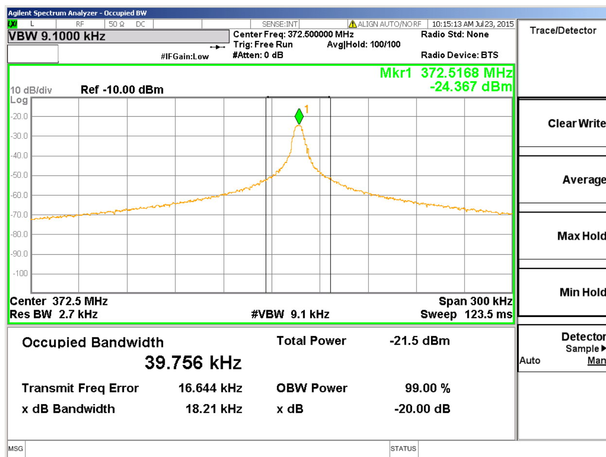
Figure 58 – 99% Bandwidth Graph
