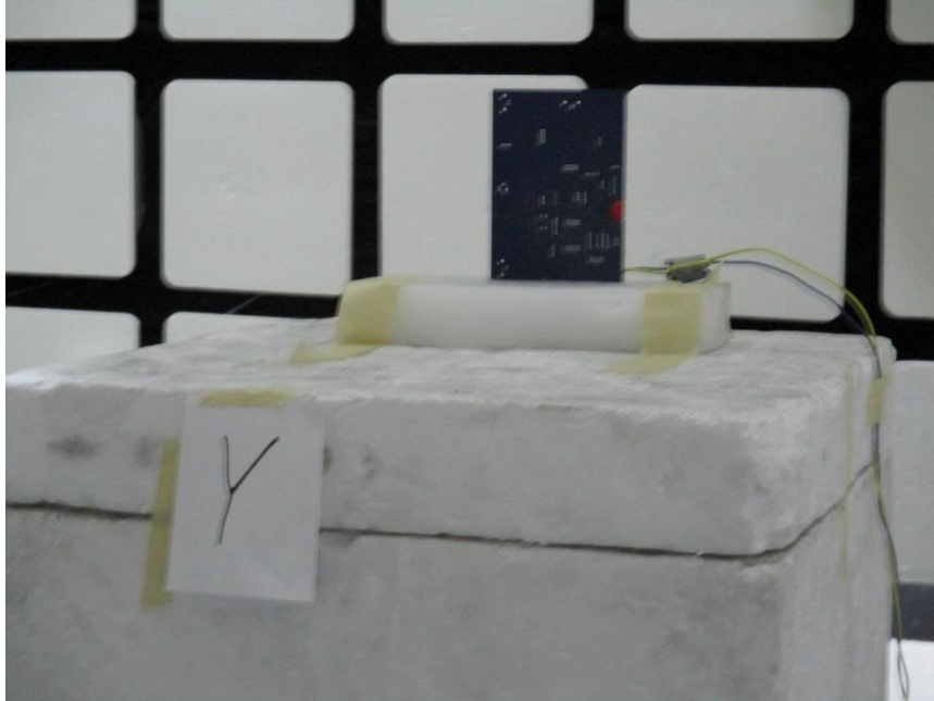
Y-AXIS SETUP
