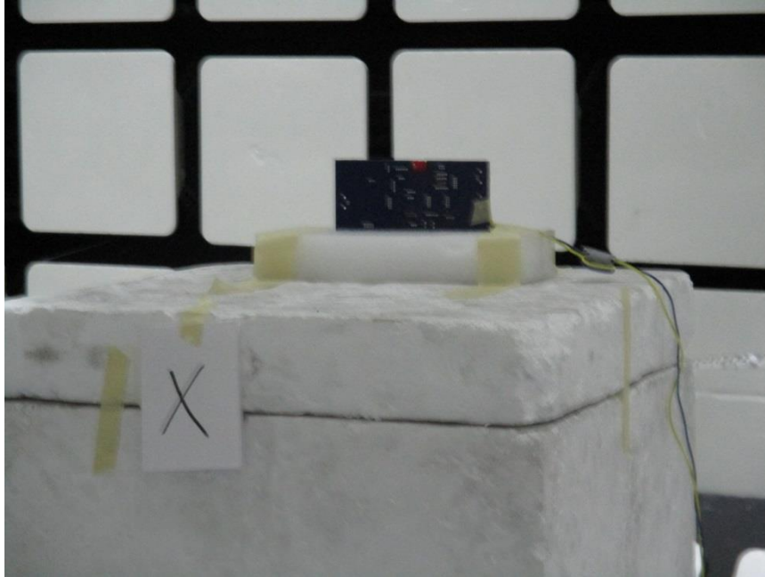
X-AXIS SETUP
