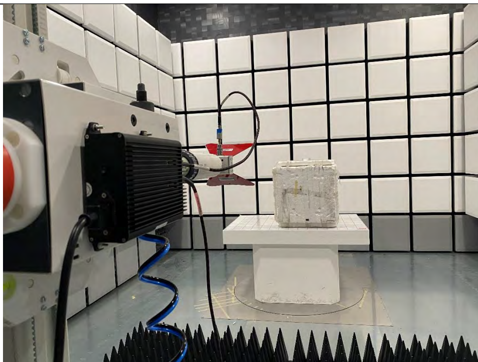
Radiated Emission Test above 1GHz Front View
