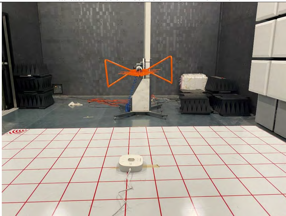
Radiated Emission Test below 1GHz Rear View
