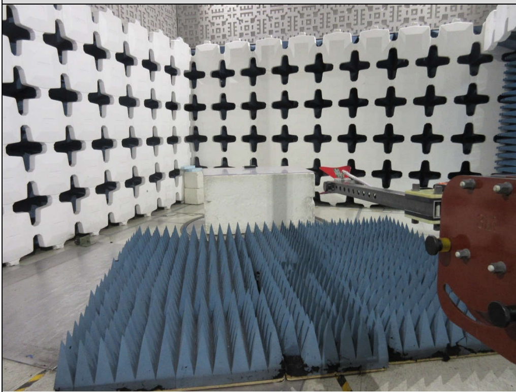
Test Setup for Radiated Emissions: 1GHz to 18GHz, Vertical Polarization
