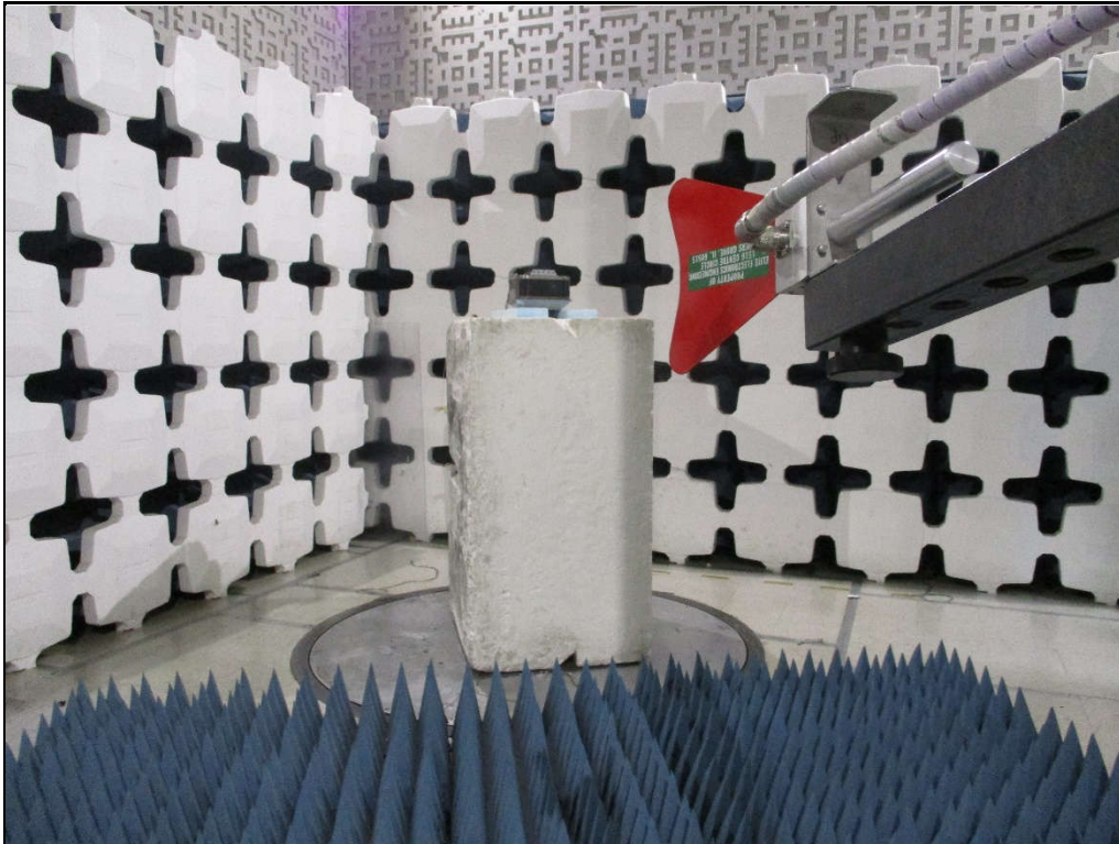
Test Setup for Spurious Radiated Emissions, 1GHz to 10GHz – Antenna Polarization Horizontal
