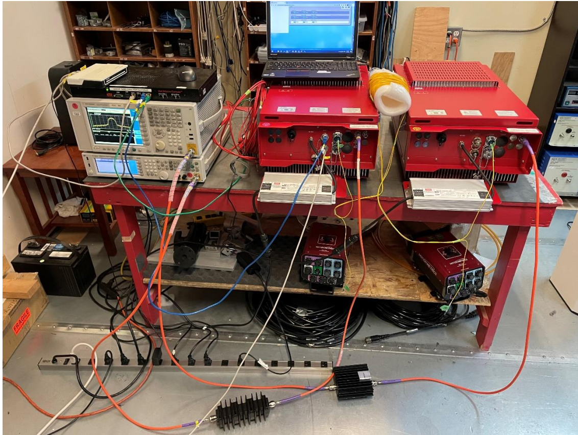
Figure 1: RF Conducted measurement Test Setup
