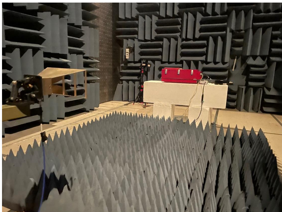
Figure 3: Radiated Emissions (Above 1GHz) Emissions Test Setup
