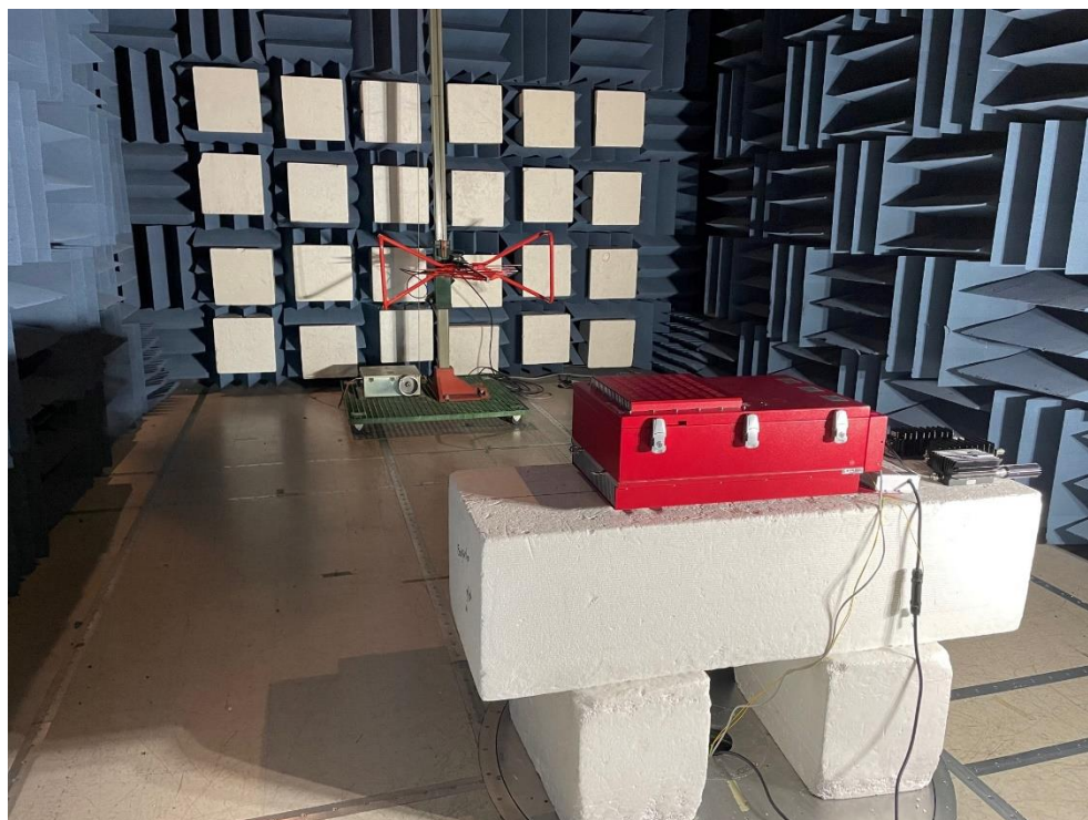
Figure 2: Radiated Emissions (Below 1GHz) Emissions Test Setup
