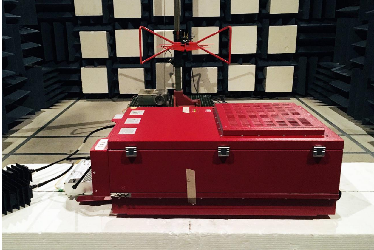
Figure 1: Radiated Emissions (Below 1GHz) Test Setup
