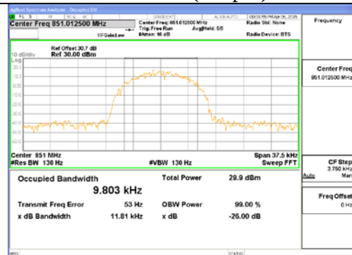
P25 II-DP (Output)
