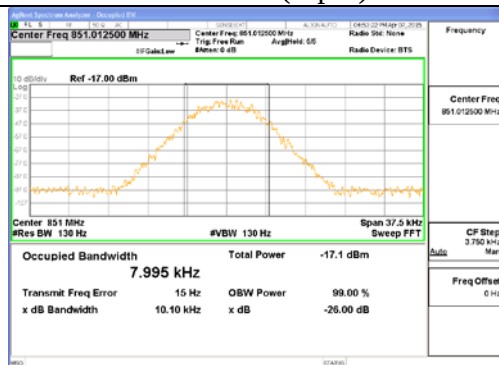
P25 II-DP (Input)
