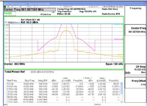
P25 II-DP on 861.9875 MHz
