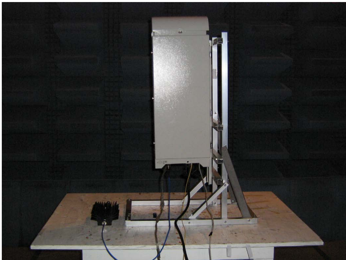
Picture 2: Radiated Emission test setup in Semi Anechoic Chamber
