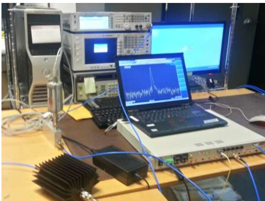
Figure 2 Conducted Test Setup – Measurement Instruments
