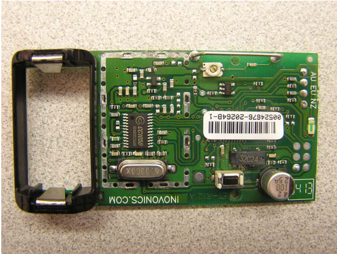
PCB top side with shield can removed
