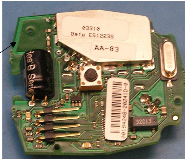
PCB Topside
