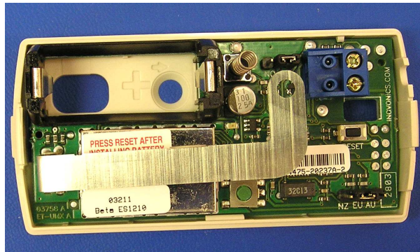
PCB Topside
