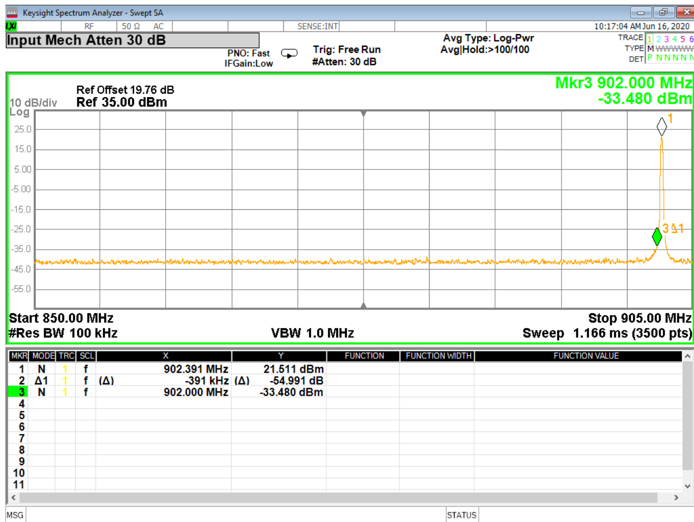
Figure 16 - Band-edge Measurement, Low Channel, Fundamental, Continuous The plot shows an uncorrected measurement, used for relative measurements only.
