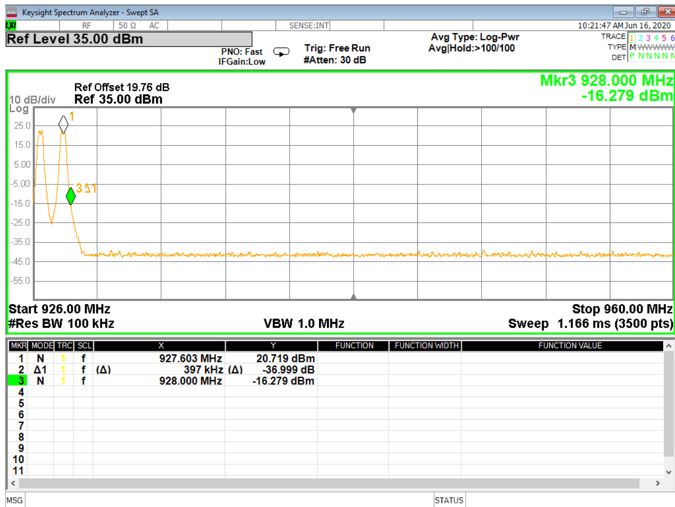
Figure 21 - Band-edge Measurement, High Channel, Fundamental, Hopping Transmit
