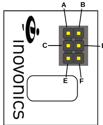
Figure 2 OEM connector pinout
