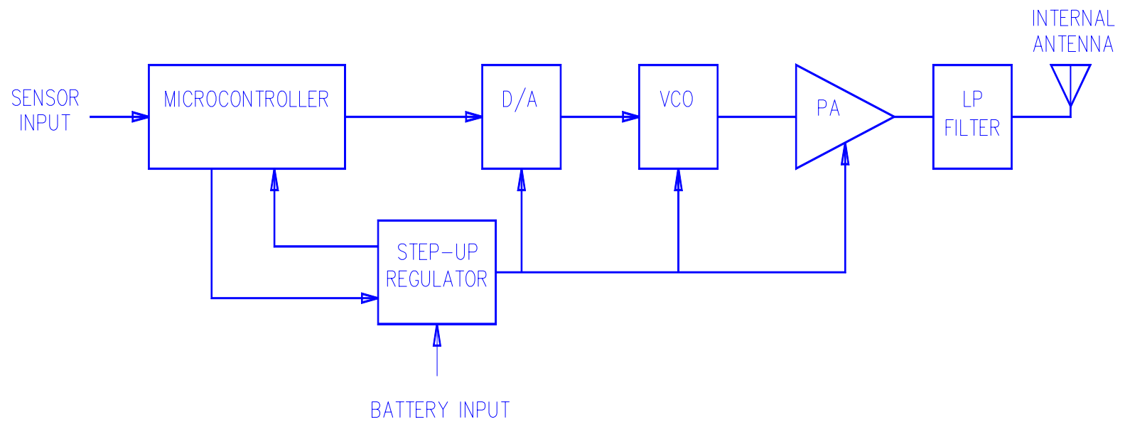
FA SERIES TRANSMITTER BLOCK DIAGRAM
