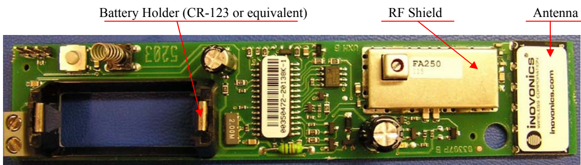
Photograph of an FA-250M board with the shield in place. Note PC mounted antenna is at the far right end of the board.
