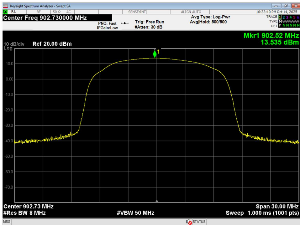
01 Conducted Peak Power, Low
