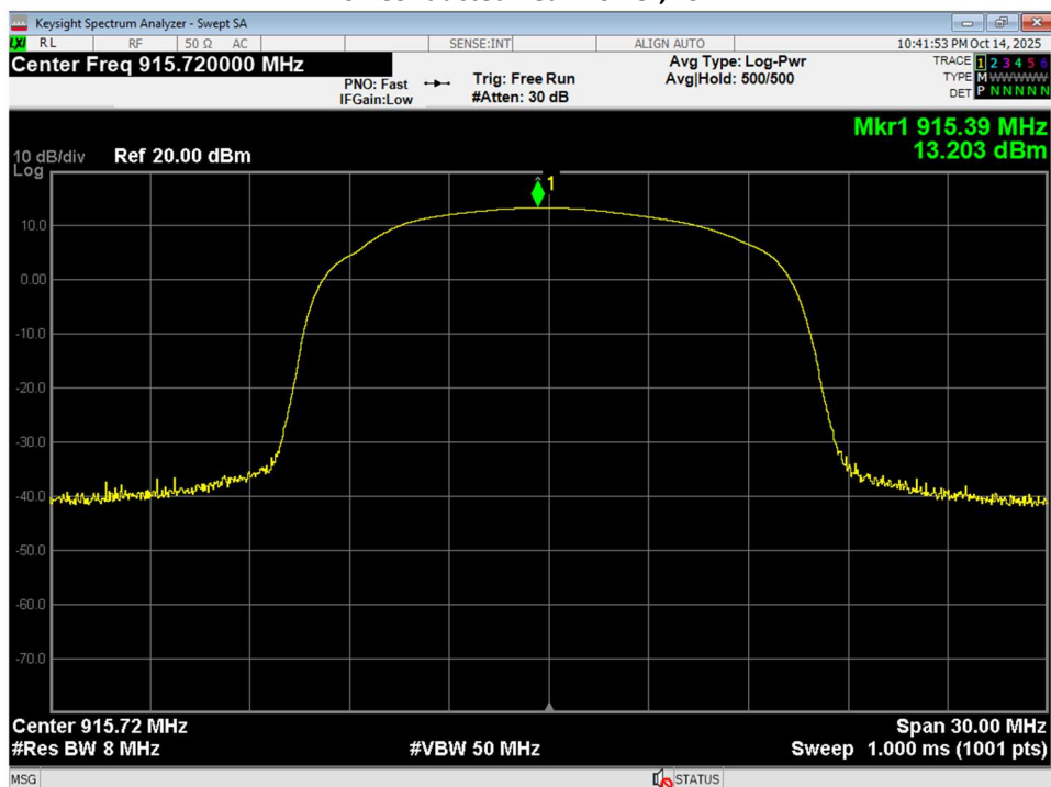
02 Conducted Peak Power, Mid
