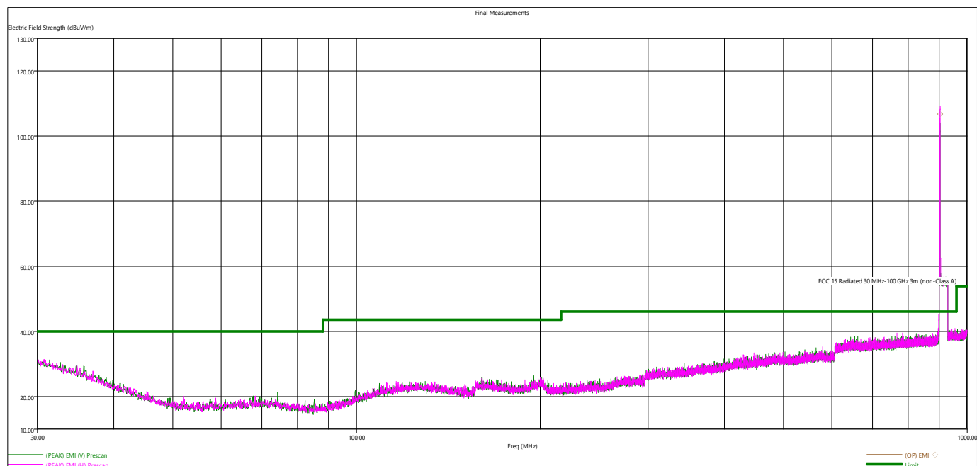
Figure 5 - Radiated Emissions Plot, Low Channel, 30M-1GHz
