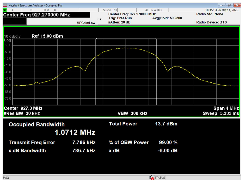
06 6dB Bandwidth, High
