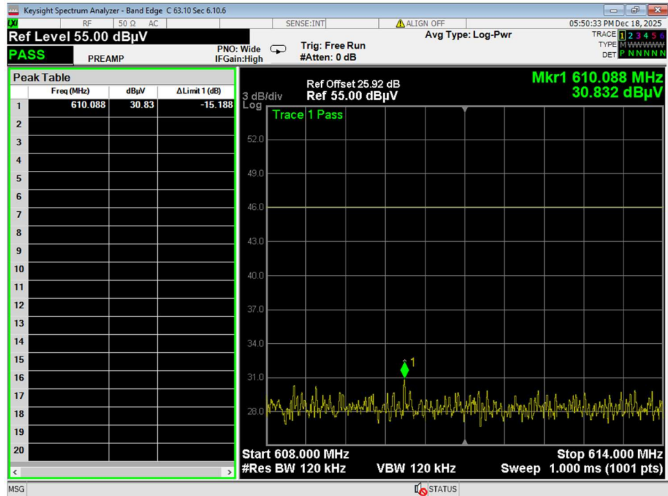
12 Lower Bandedge, Restricted
