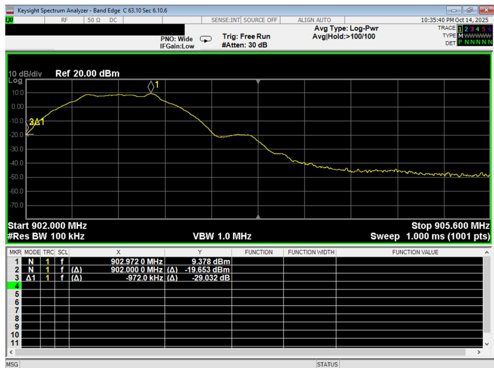
10 Lower Bandedge, Unrestricted
