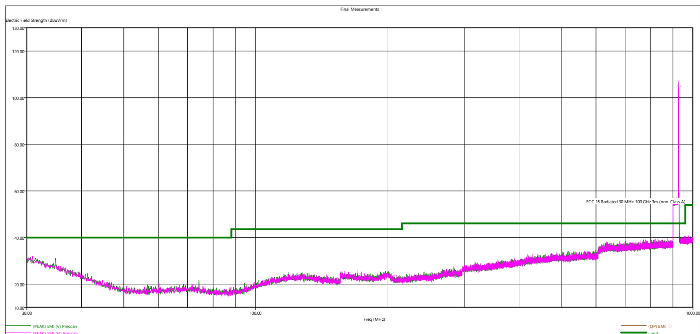
Figure 7 - Radiated Emissions Plot, High Channel, 30M-1GHz
