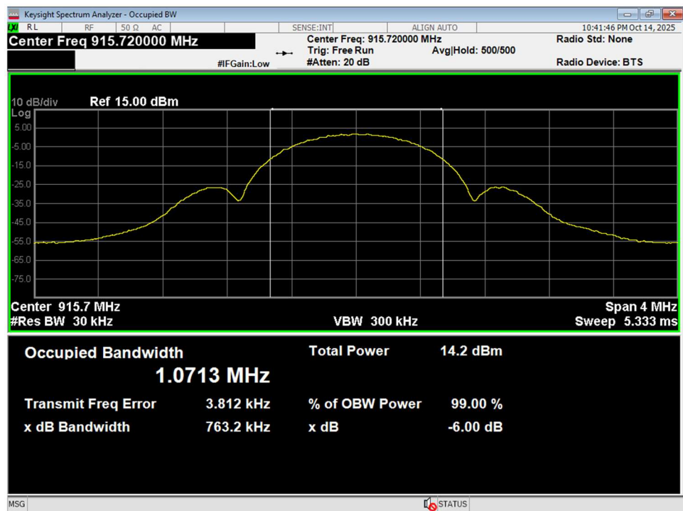
05 6dB Bandwidth, Mid
