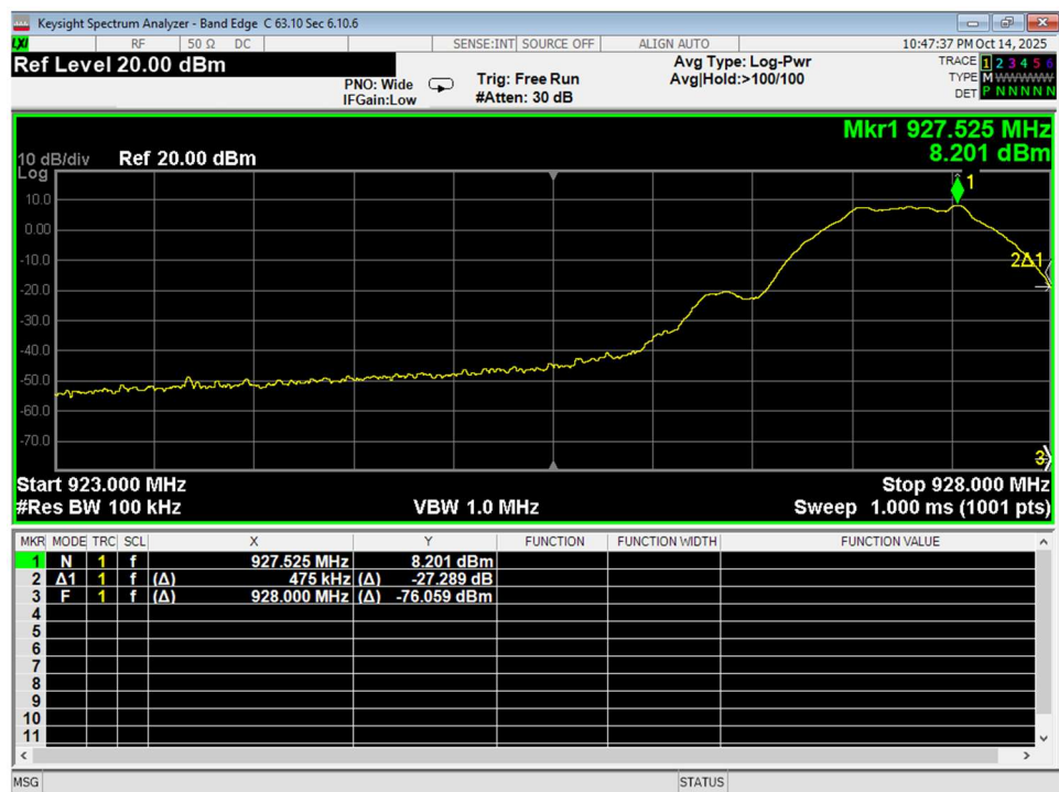
11 Higher Bandedge, Unrestricted
