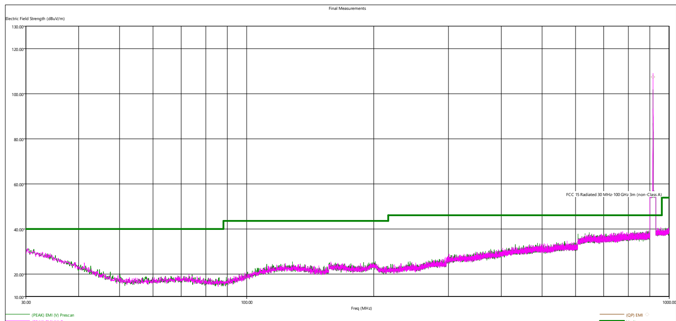
Figure 6 - Radiated Emissions Plot, Mid Channel, 30M-1GHz
