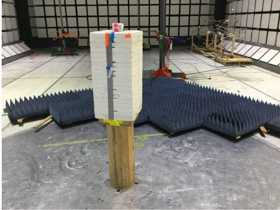
Radiated Emissions, 1GHz – 18GHz
