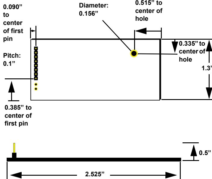
Figure 3 One-way serial RF module dimensions
