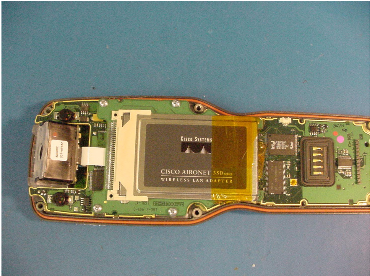
PHOTOGRAPH 7: WLAN LOCATION IN EUT COMPTUER
